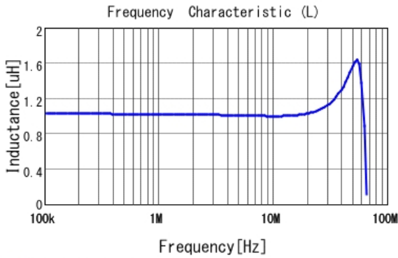
■ 1239AS-H-1R0M L
