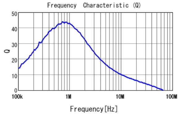
■ 1239AS-H-1R0M Q
