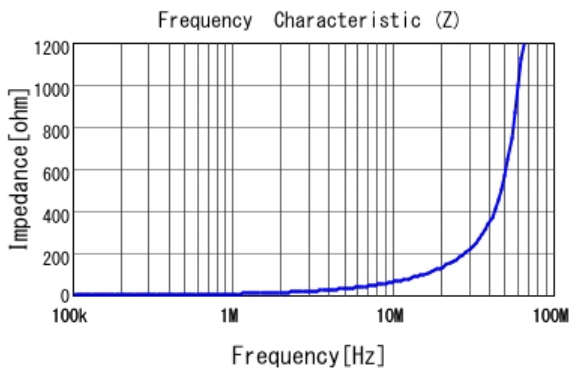
■ 1239AS-H-1R0M |Z|
